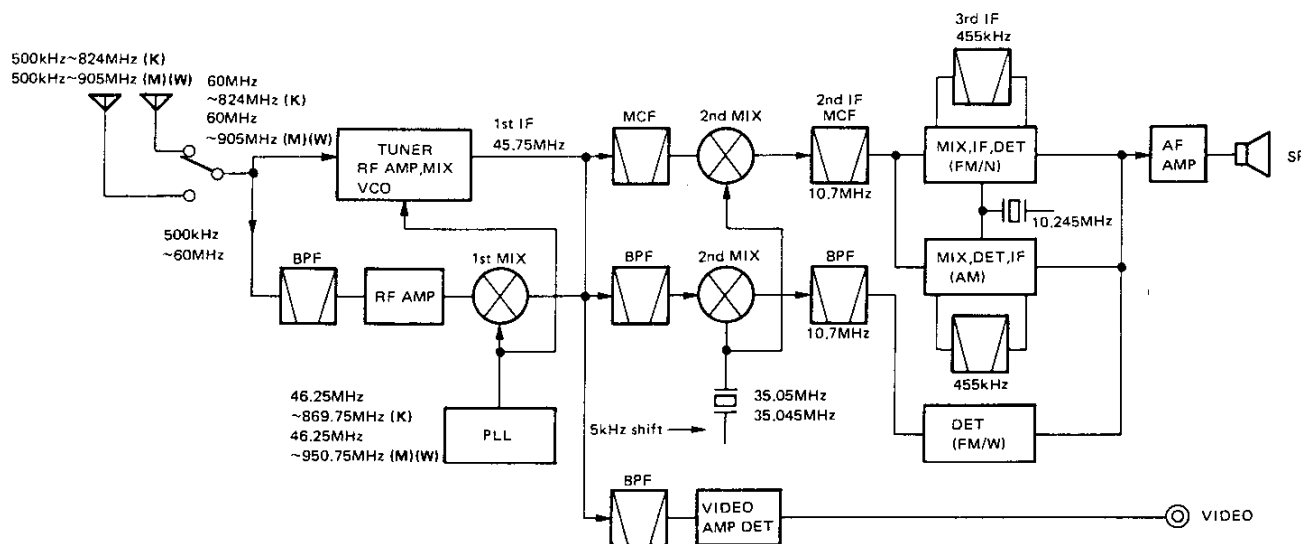
Fig. 2 Frequency configuration
