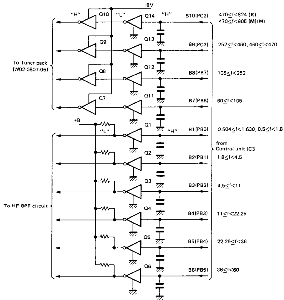
Fig. 9 Band information circuit
