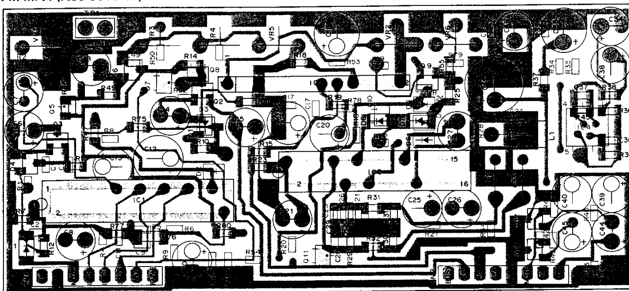
FM MPX (X58-3310-11) Foil side view
